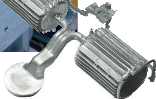
Aluminium pump housing fixed to the filling system, i.e. runners, gates and overflows.
