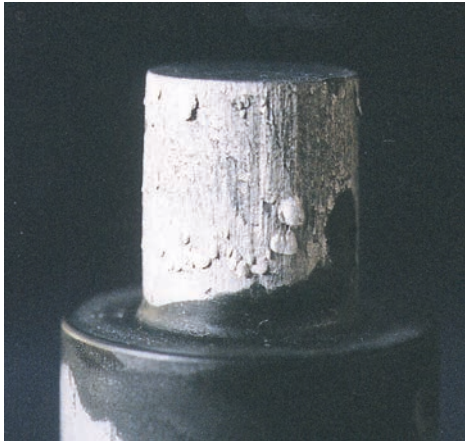
Soldering damage on a core pin.
